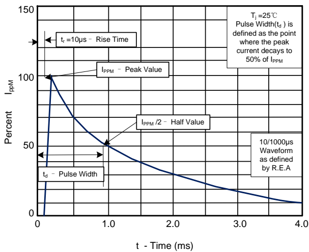
Figure 3. Pulse Waveform
